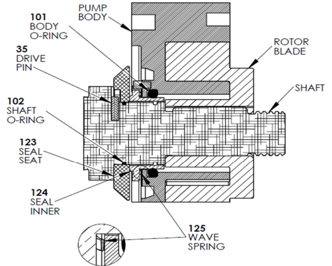
SINGLE MECHANICAL SEAL
