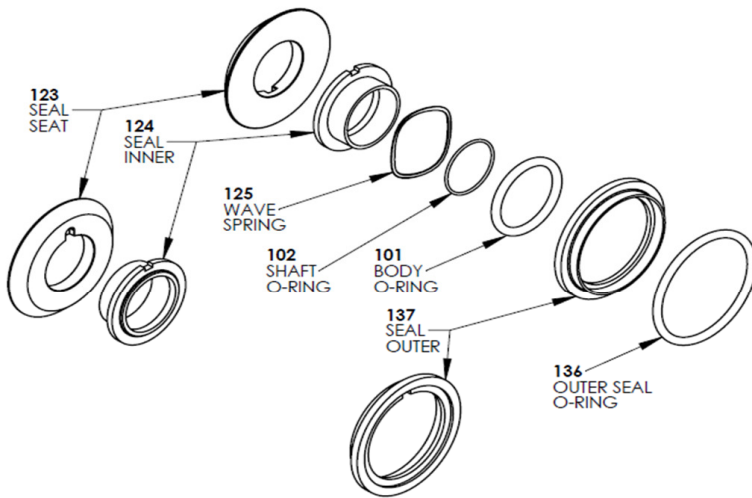
ZP1 DOUBLE MECHANICAL SEAL PARTS
