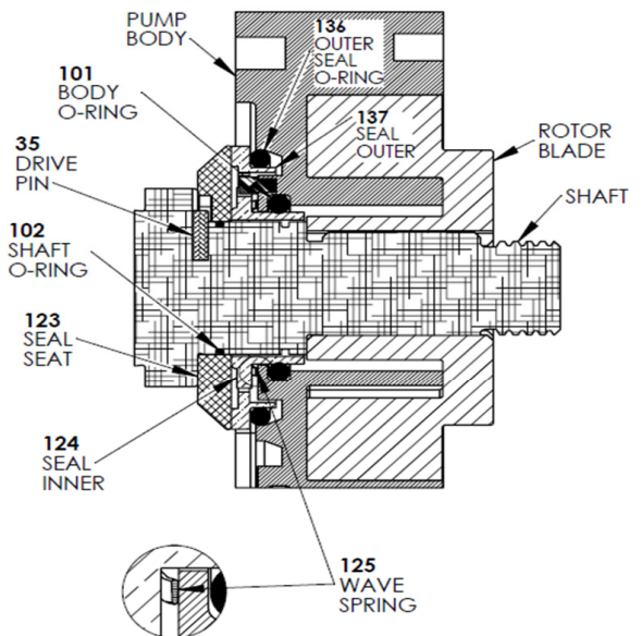
DOUBLE MECHANICAL SEAL
