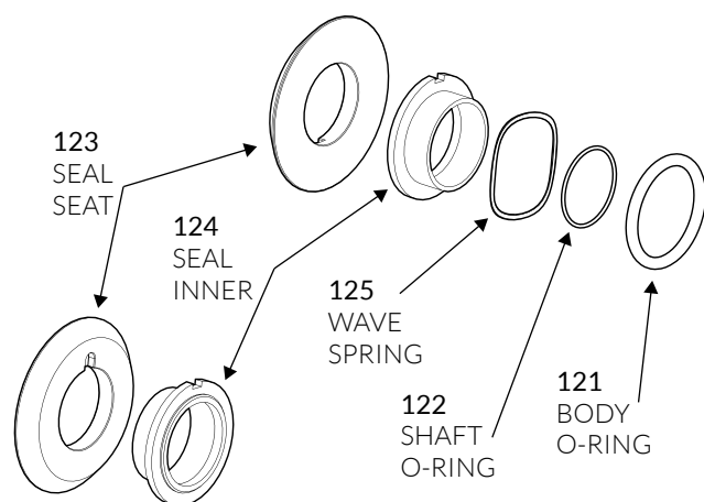
SINGLE MECHANICAL SEAL PARTS
