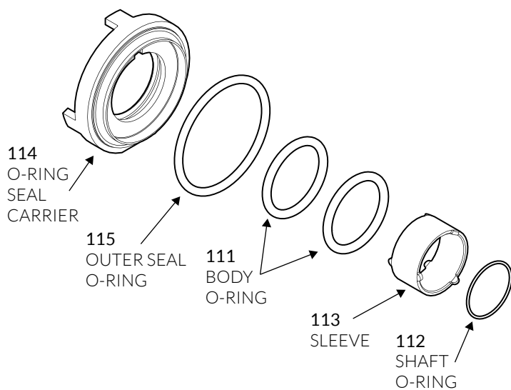
DOUBLE O-RING SEAL PARTS
