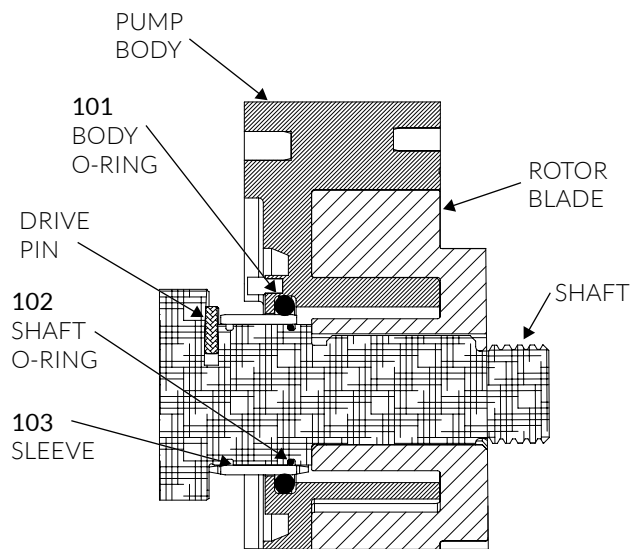
SINGLE O-RING SEAL
