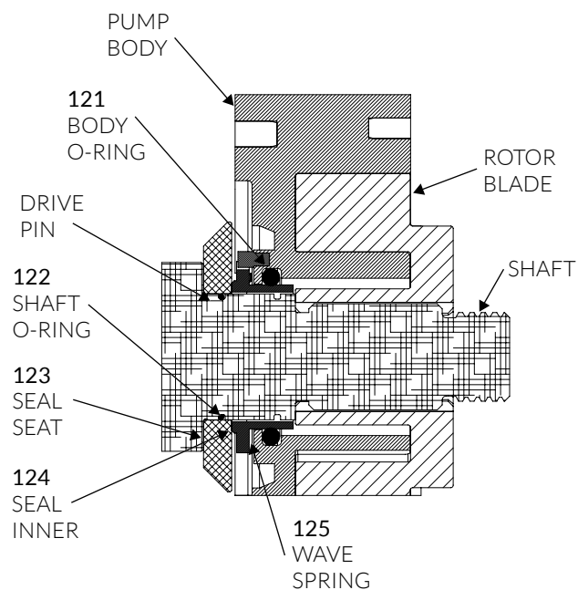
SINGLE MECHANICAL SEAL
