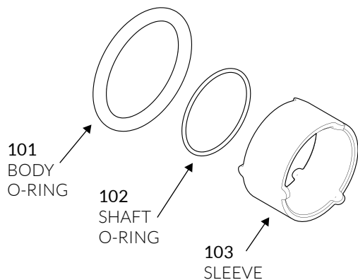
SINGLE O-RING SEAL PARTS
