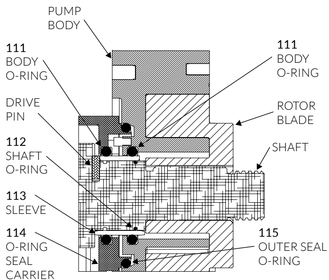
DOUBLE O-RING SEAL
