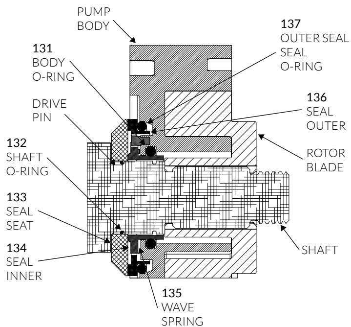
DOUBLE MECHANICAL SEAL
