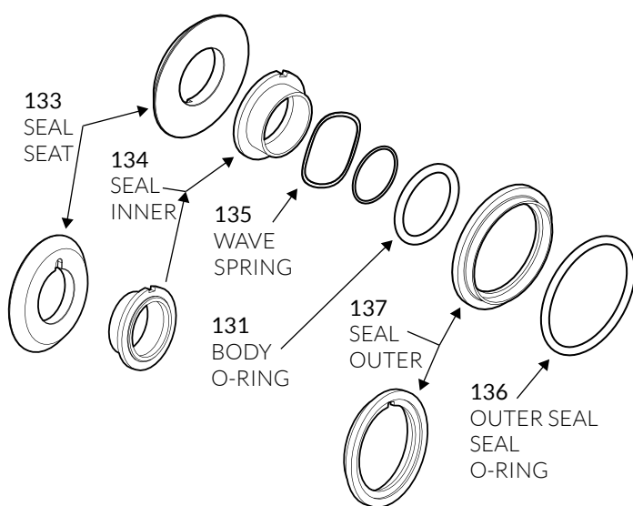
DOUBLE MECHANICAL SEAL PARTS
