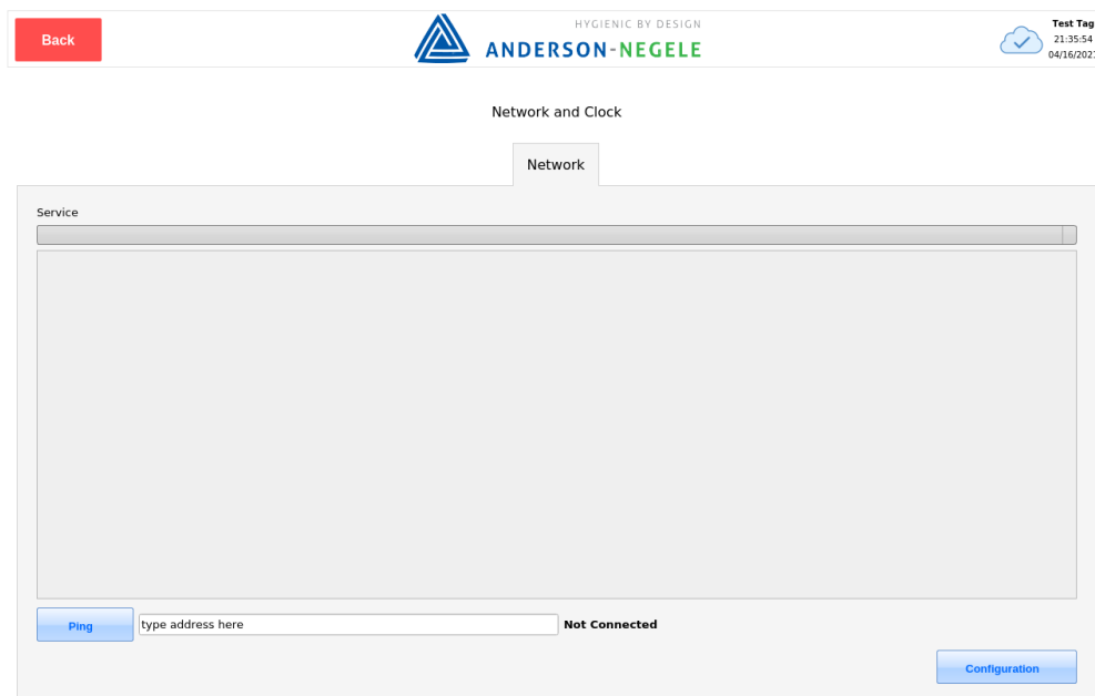
Figure 68: Ping Feature
