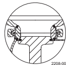
Figure 4. Replaceable elastomer plug seal
