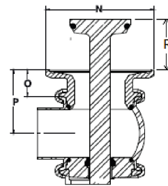
Figure 3. Flange adapter
