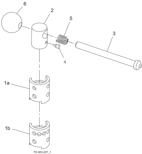
Handle 1.1 with infinite positions for LKB Butterfly valve
