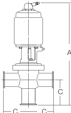
771-30 Shut-Off Valve
