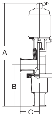
771-27 Reverse-Acting Valve
