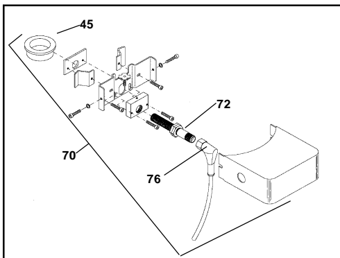
2" Bracket
