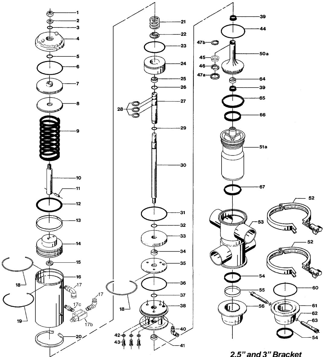
2.5" and 3" Bracket
