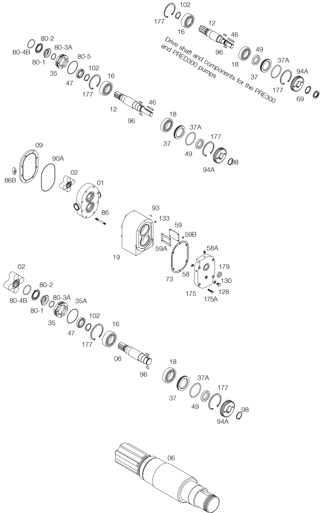
Pump shaft for PRE300 and PRED pumps
