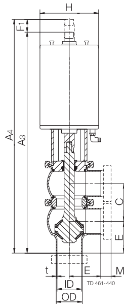
Change-over valve
