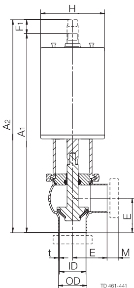
Shut-off valve
